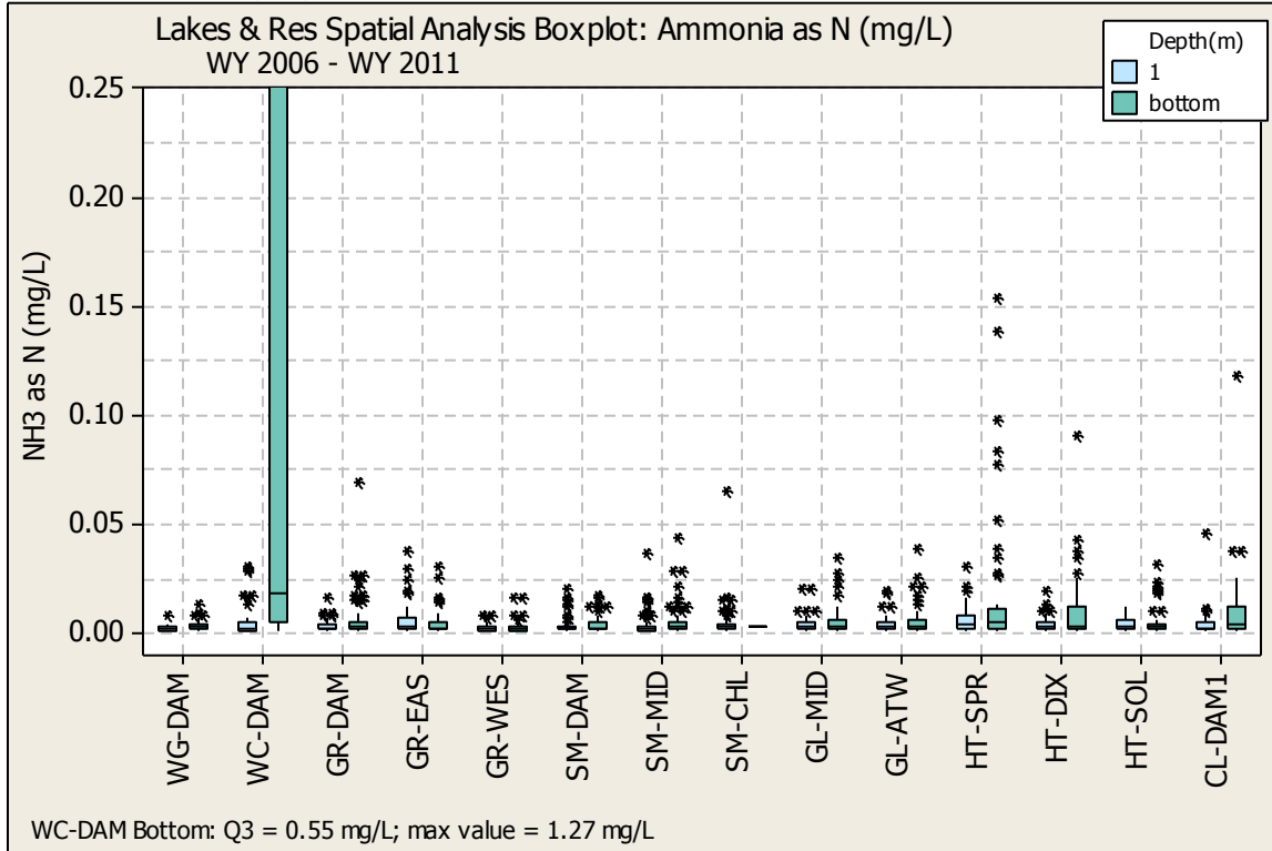
Figure E.3 AMMONIA (NH3) SPATIAL ANALYSIS BOX PLOT
