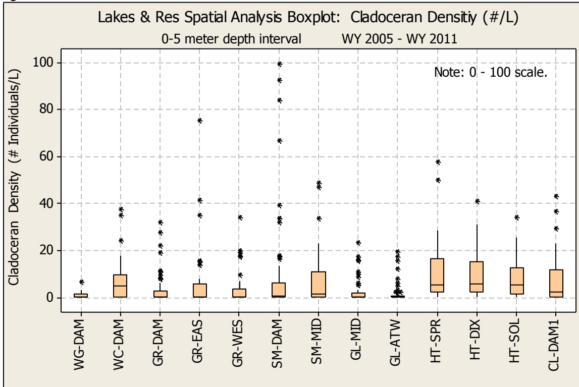
Figure E. 39 CLADOCERAN DENSITY SPATIAL ANALYSIS BOX PLOT
