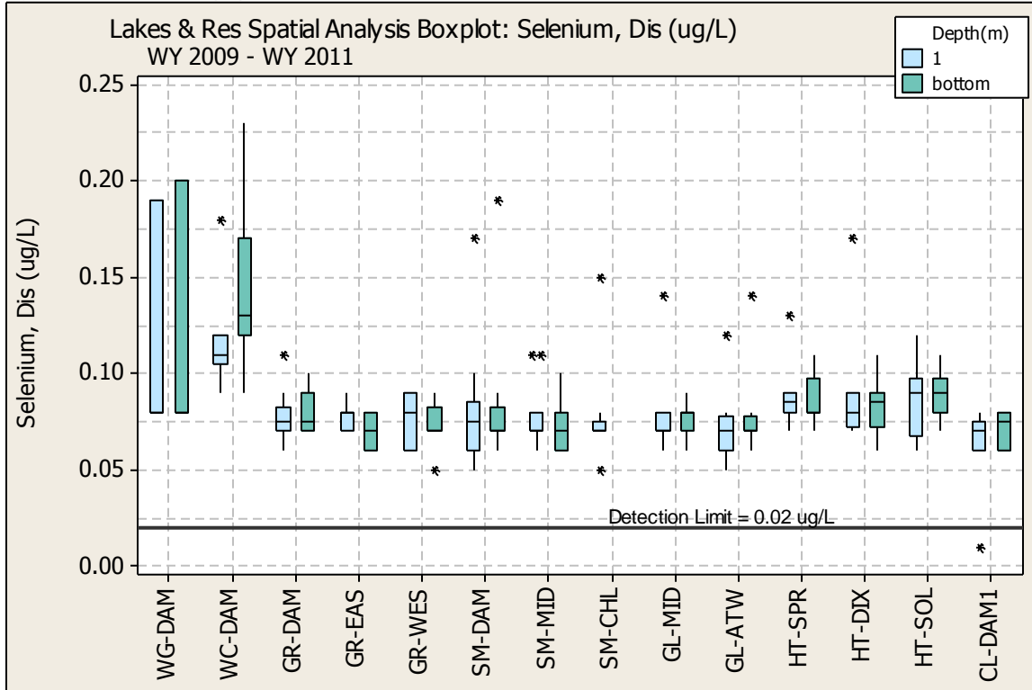
Figure E. 27 SELENIUM (Se) SPATIAL ANALYSIS BOX PLOT
