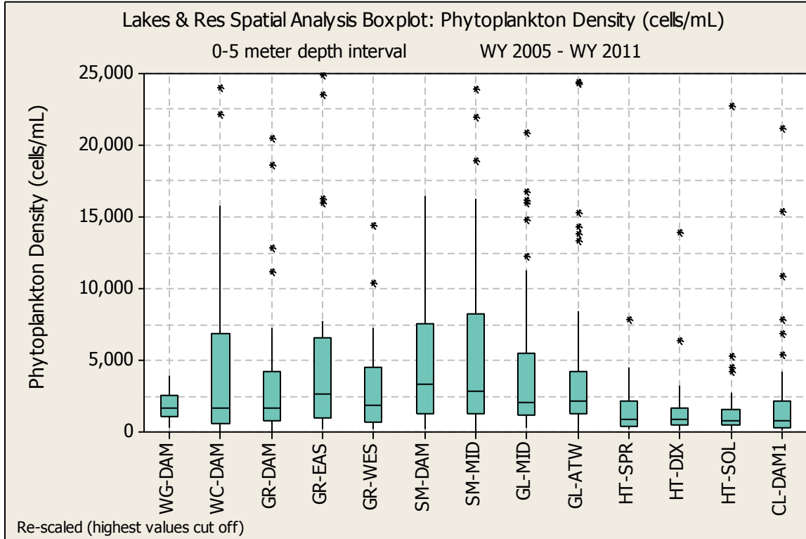
Figure E. 31 PHYTOPLANKTON DENSITY SPATIAL ANALYSIS BOX PLOT -- RESCALED
