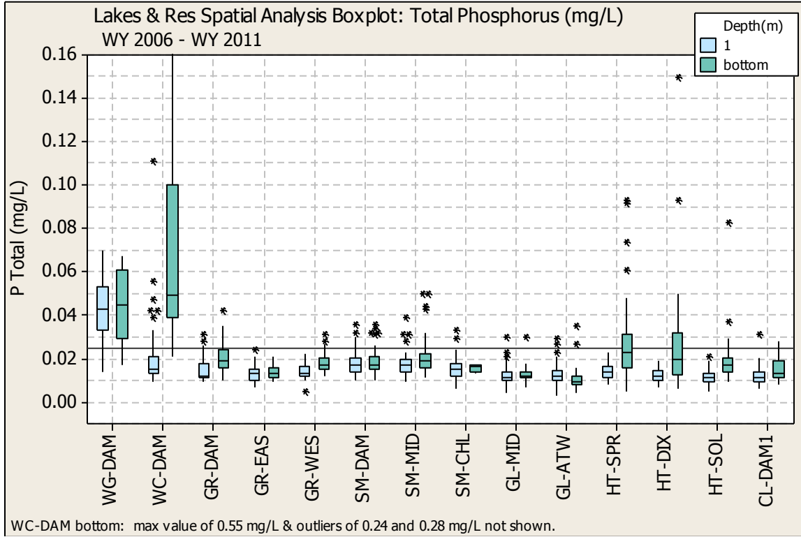
Figure E. 7 TOTAL PHOSPHORUS (TP) SPATIAL ANALYSIS BOX PLOT
