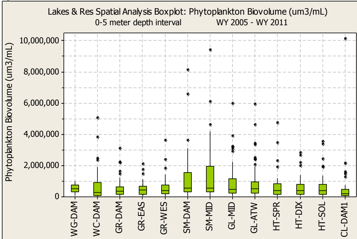
Figure E. 32 PHYTOPLANKTON BIOVOLUME SPATIAL ANALYSIS BOX PLOT
