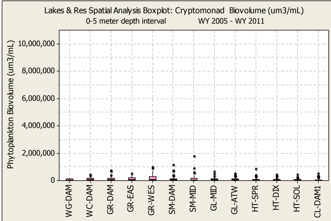
Figure E. 35 CRYPTOMONAD BIOVOLUME SPATIAL ANALYSIS BOX PLOT
