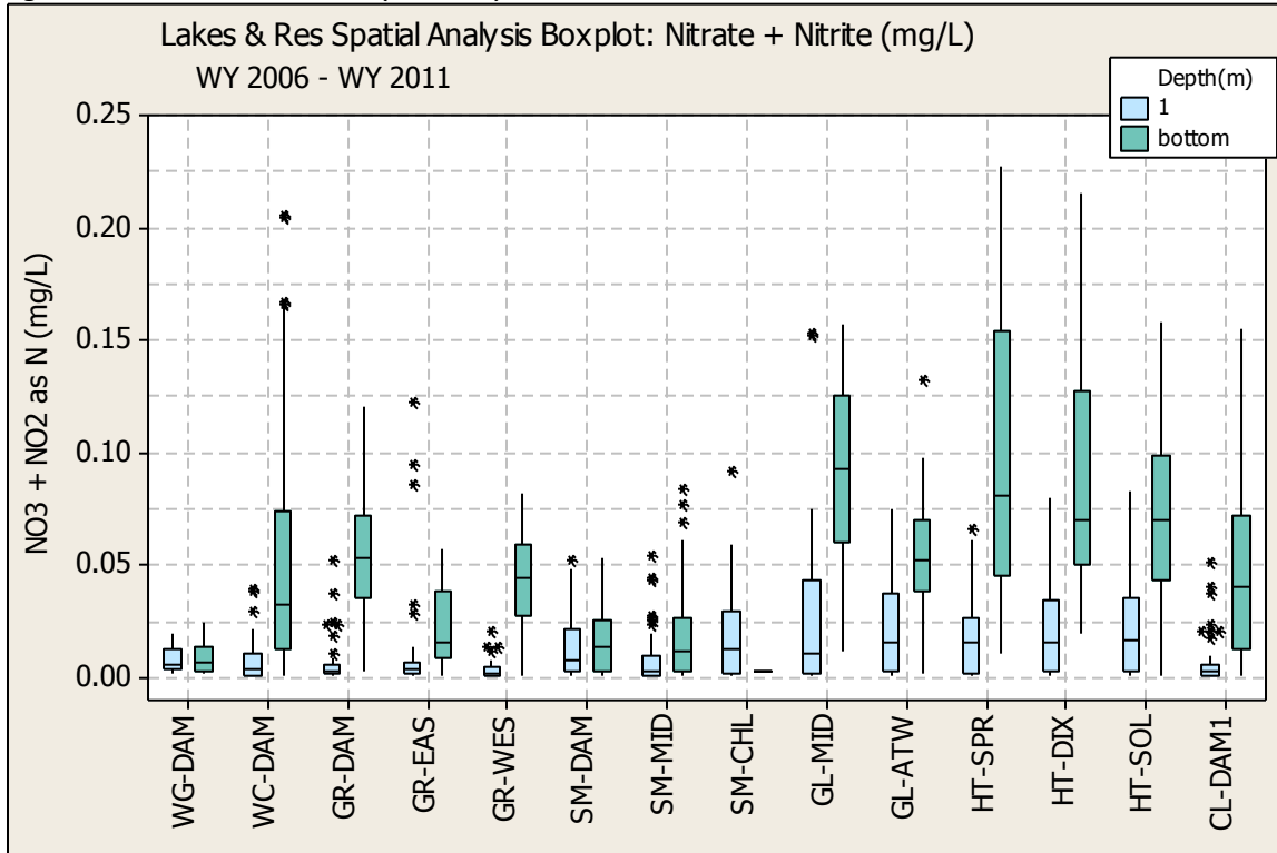
Figure E.4 NITRATE PLUS NITRITE (NO3+NO2) SPATIAL ANALYSIS BOX PLOT
