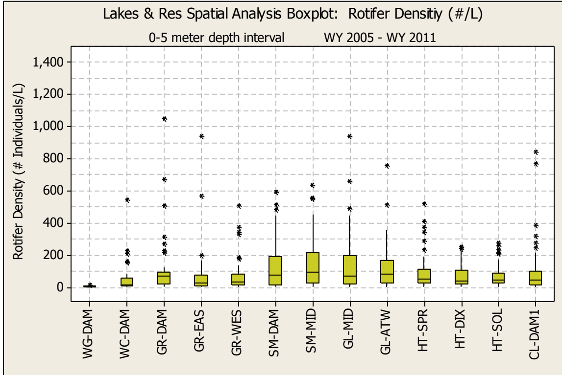
Figure E. 37 ROTIFER DENSITY SPATIAL ANALYSIS BOX PLOT
