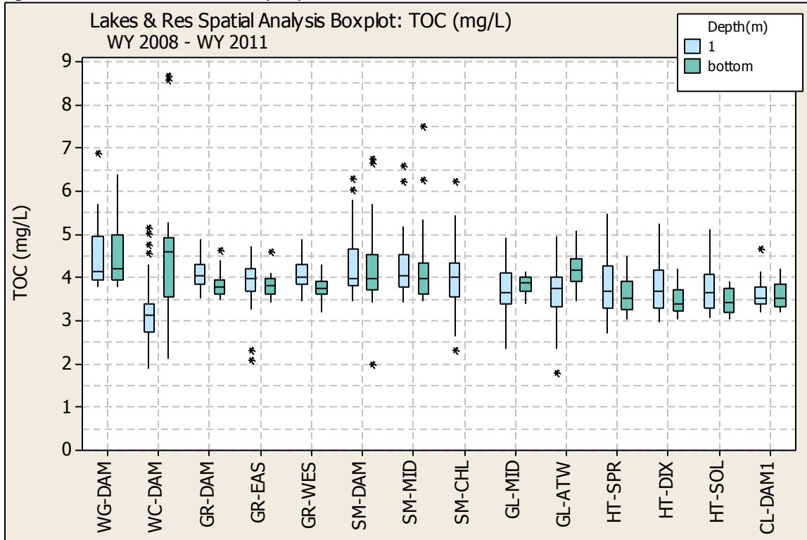
Figure E. 8 TOTAL ORGANIC CARBON (TOC) SPATIAL ANALYSIS BOX PLOT
