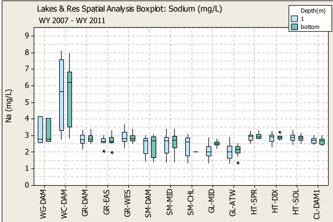
Figure E. 13 SODIUM (Na) SPATIAL ANALYSIS BOX PLOT
