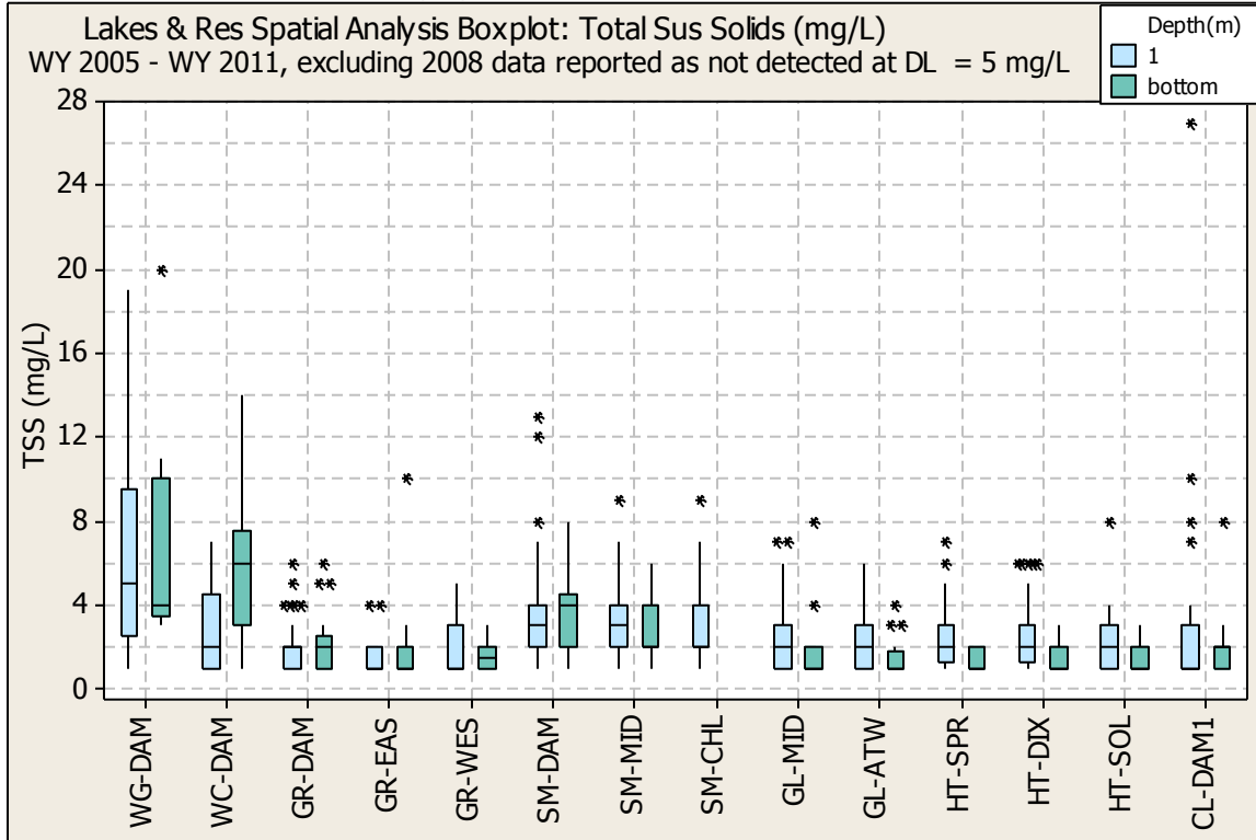
Figure E. 9 TOTAL SUSPENDED SOLIDS (TSS) SPATIAL ANALYSIS BOX PLOT
