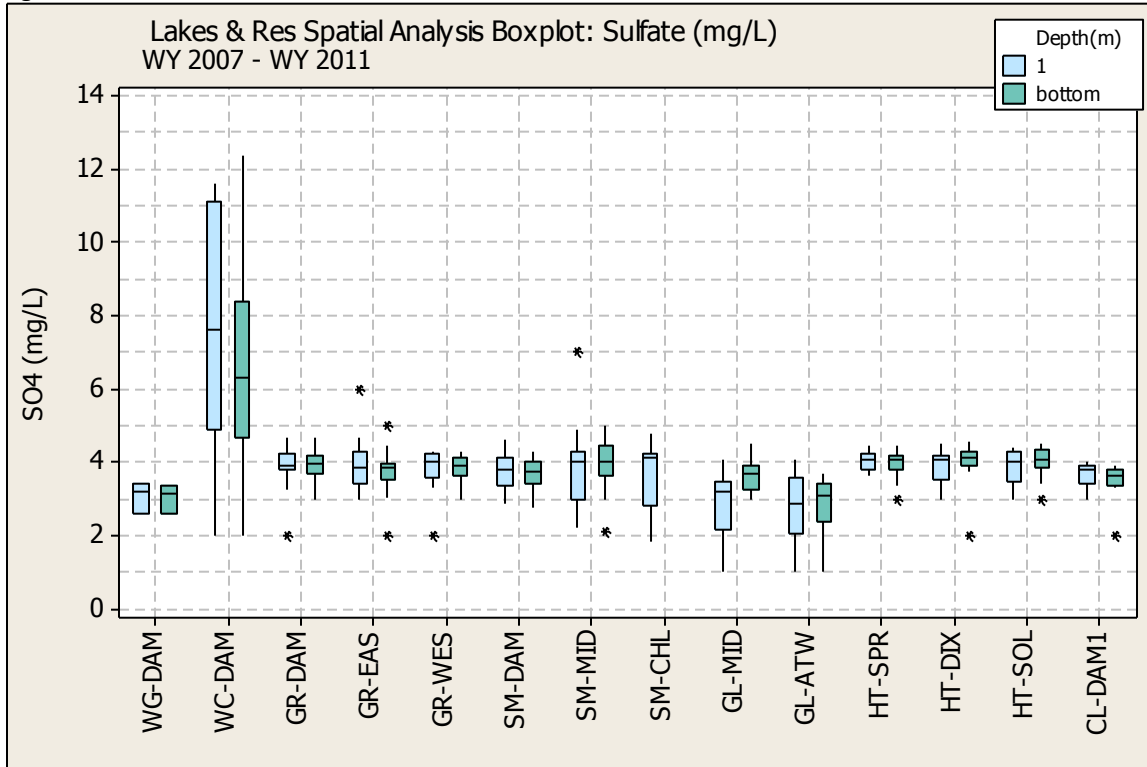
Figure E. 16 SULFATE SPATIAL ANALYSIS BOX PLOT
