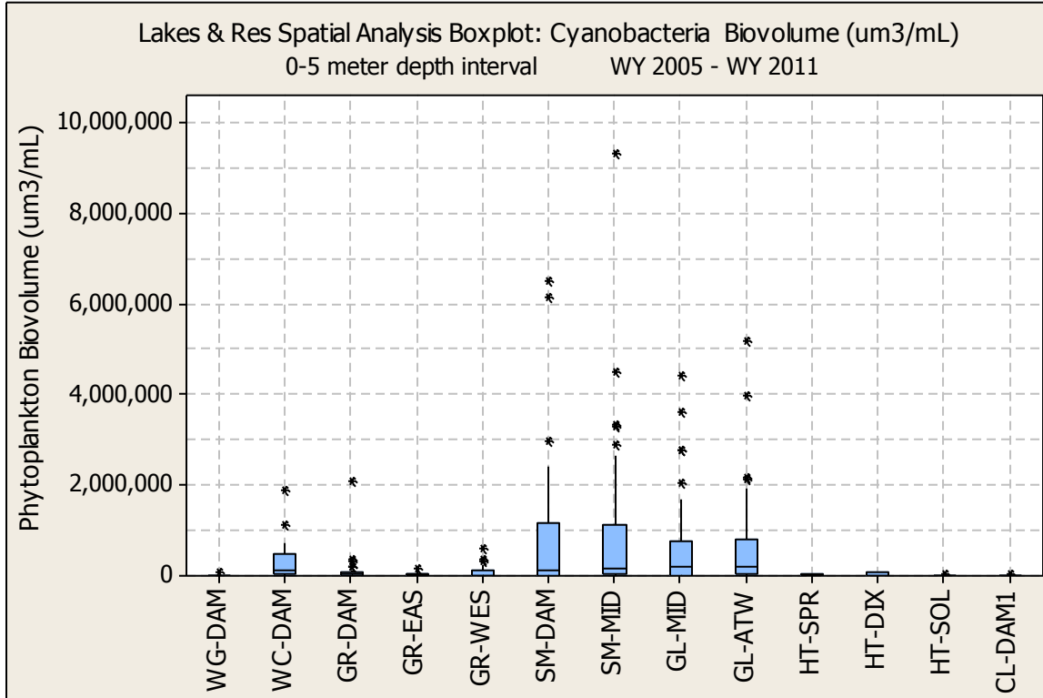
Figure E. 33 CYANOBACTERIA BIOVOLUME SPATIAL ANALYSIS BOX PLOT
