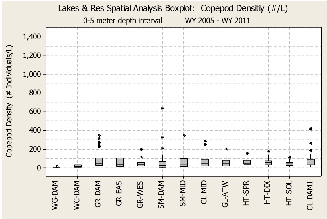
Figure E. 38 COPEPOD DENSITY SPATIAL ANALYSIS BOX PLOT
