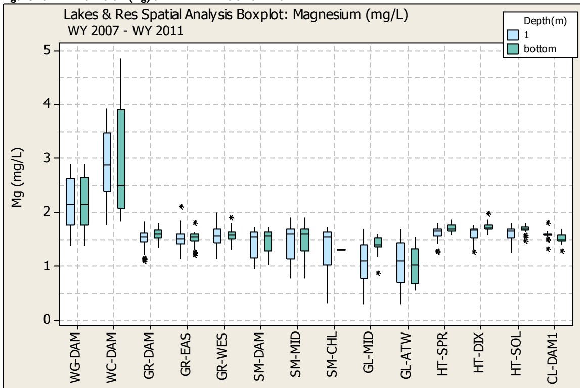
Figure E. 12 MAGNESIUM (Mg) SPATIAL ANALYSIS BOX PLOT
