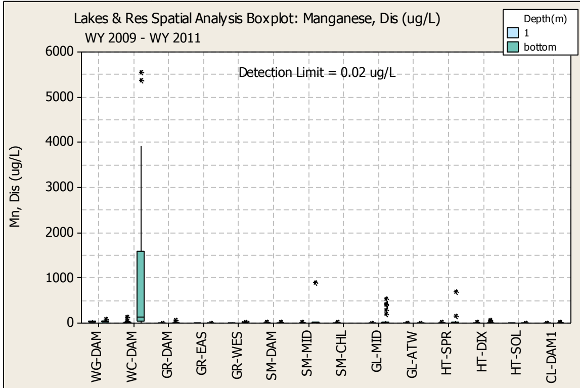
Figure E. 23 MANGANESE (Mn) SPATIAL ANALYSIS BOX PLOT
