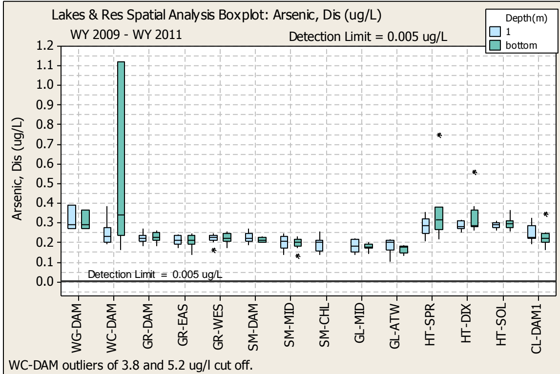
Figure E. 17 ARSENIC (As) SPATIAL ANALYSIS BOX PLOT
