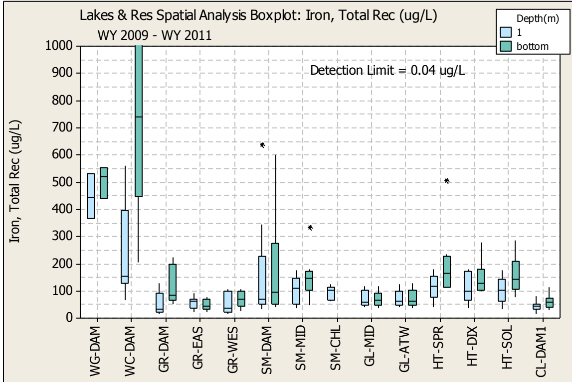
Figure E. 21 IRON (Fe), TOTAL SPATIAL ANALYSIS BOX PLOT
