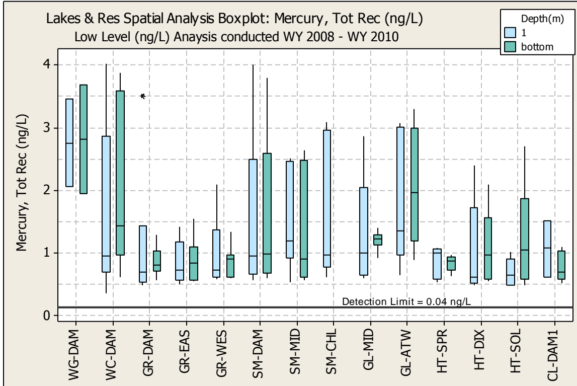
Figure E. 25 MERCURY (Hg) SPATIAL ANALYSIS BOX PLOT
