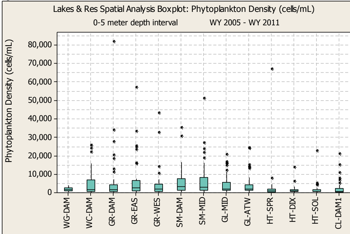
Figure E. 30 PHYTOPLANKTON DENSITY SPATIAL ANALYSIS BOX PLOT
