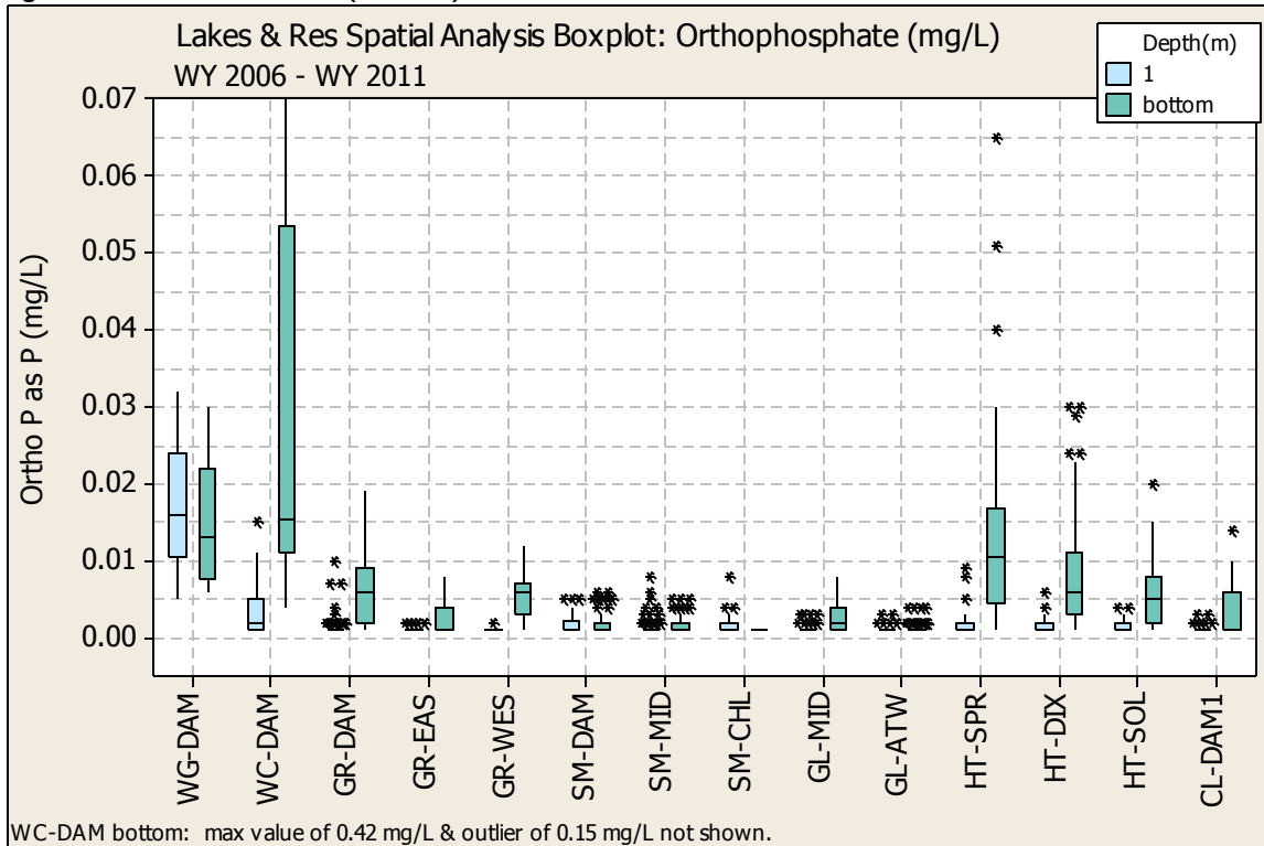
Figure E. 6 ORTHOPHOSPHATE (ORTHO-P) SPATIAL ANALYSIS BOX PLOT
