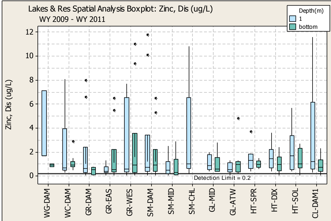
Figure E. 29 ZINC (Zn) SPATIAL ANALYSIS BOX PLOT
