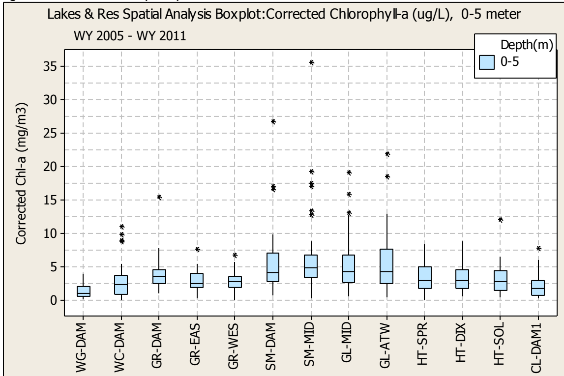
Figure E. 2 CHLOROPHYLL-A (CHL-A) SPATIAL ANALYSIS BOX PLOT
