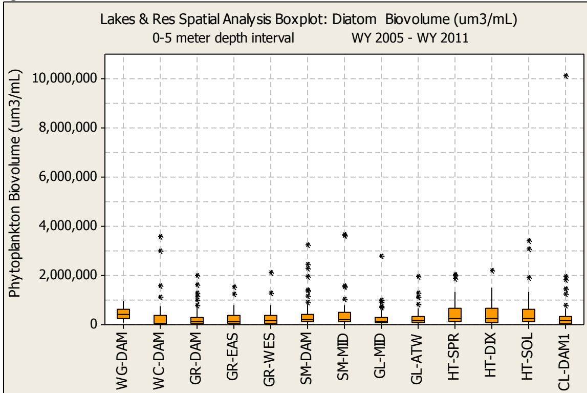
Figure E. 34 DIATOM BIOVOLUME SPATIAL ANALYSIS BOX PLOT
