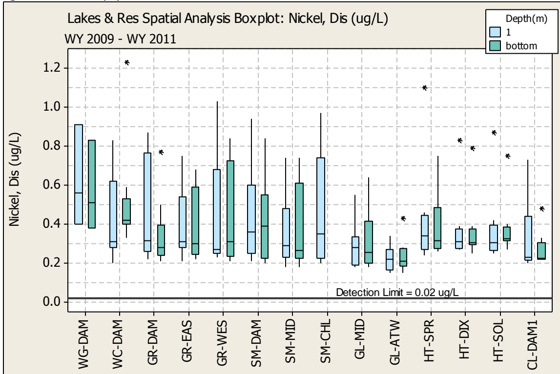
Figure E. 26 NICKEL (Ni) SPATIAL ANALYSIS BOX PLOT
