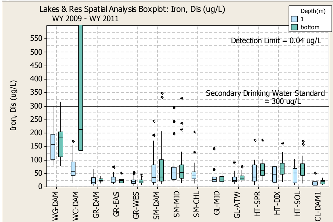
Figure E. 20 IRON (Fe) SPATIAL ANALYSIS BOX PLOT
