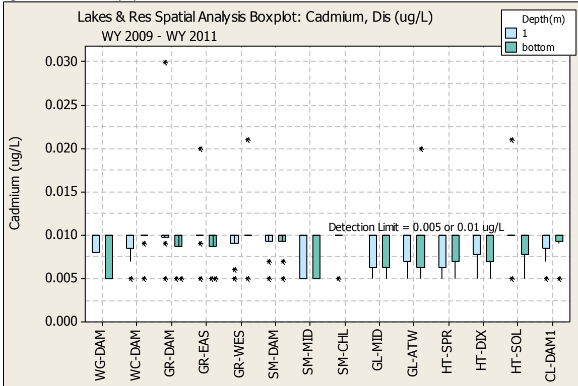
Figure E. 18 CADMIUM (Cd) SPATIAL ANALYSIS BOX PLOT
