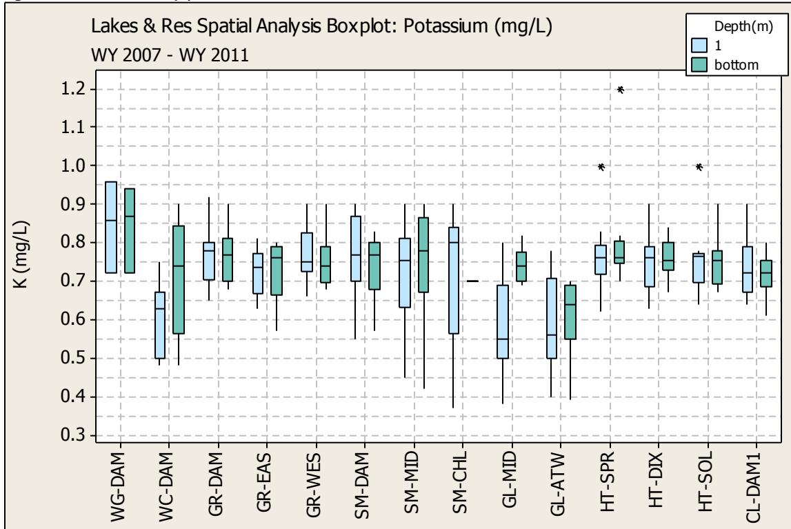
Figure E. 14 POTASSIUM (K) SPATIAL ANALYSIS BOX PLOT
