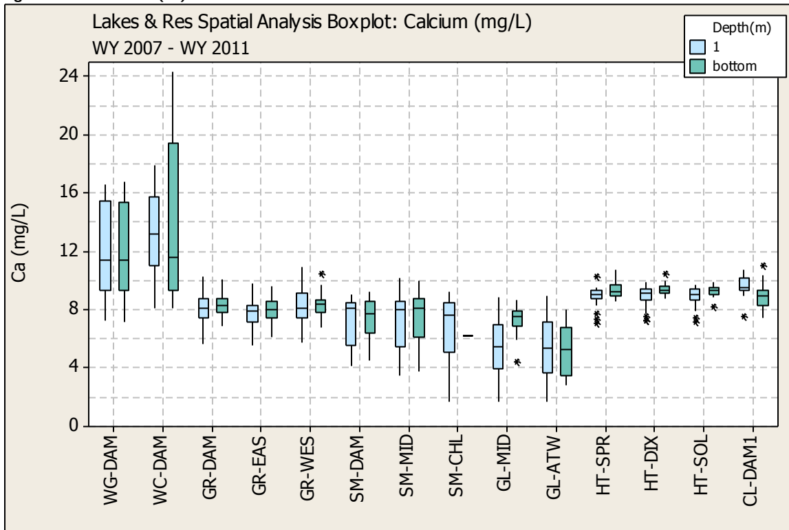
Figure E. 11 CALCIUM (Ca) SPATIAL ANALYSIS BOX PLOT
