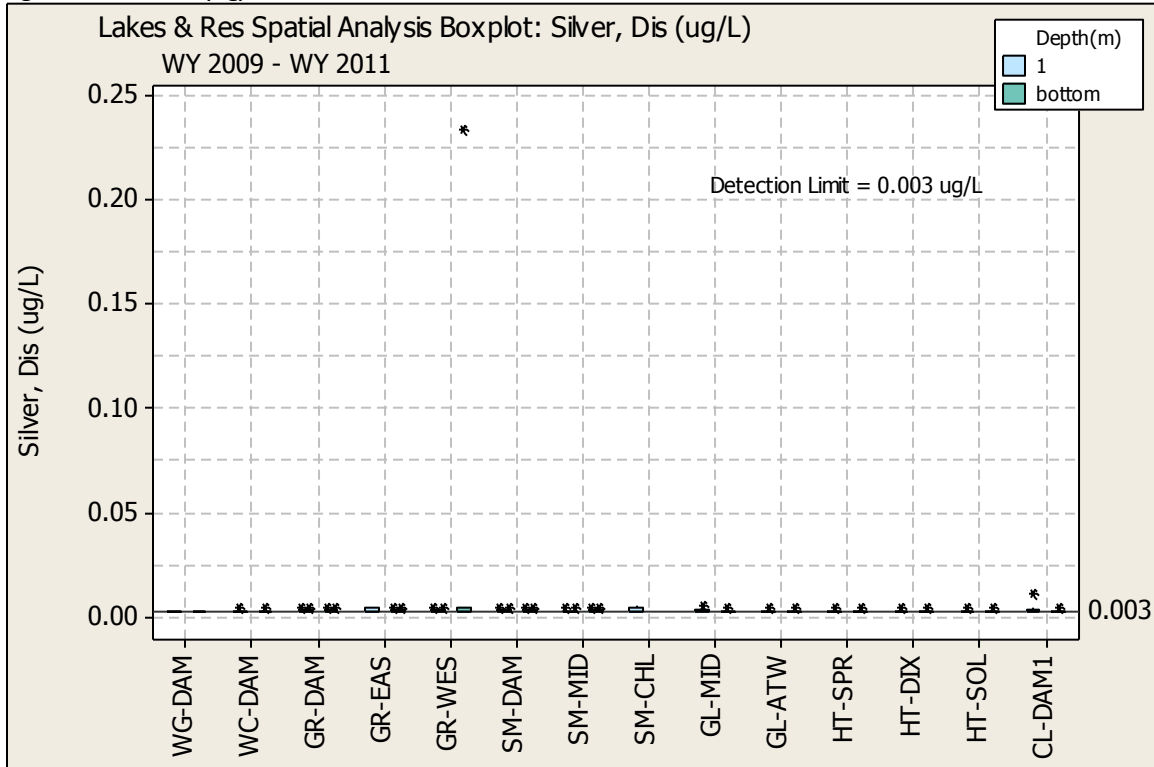
Figure E. 28 SILVER (Ag) SPATIAL ANALYSIS BOX PLOT
