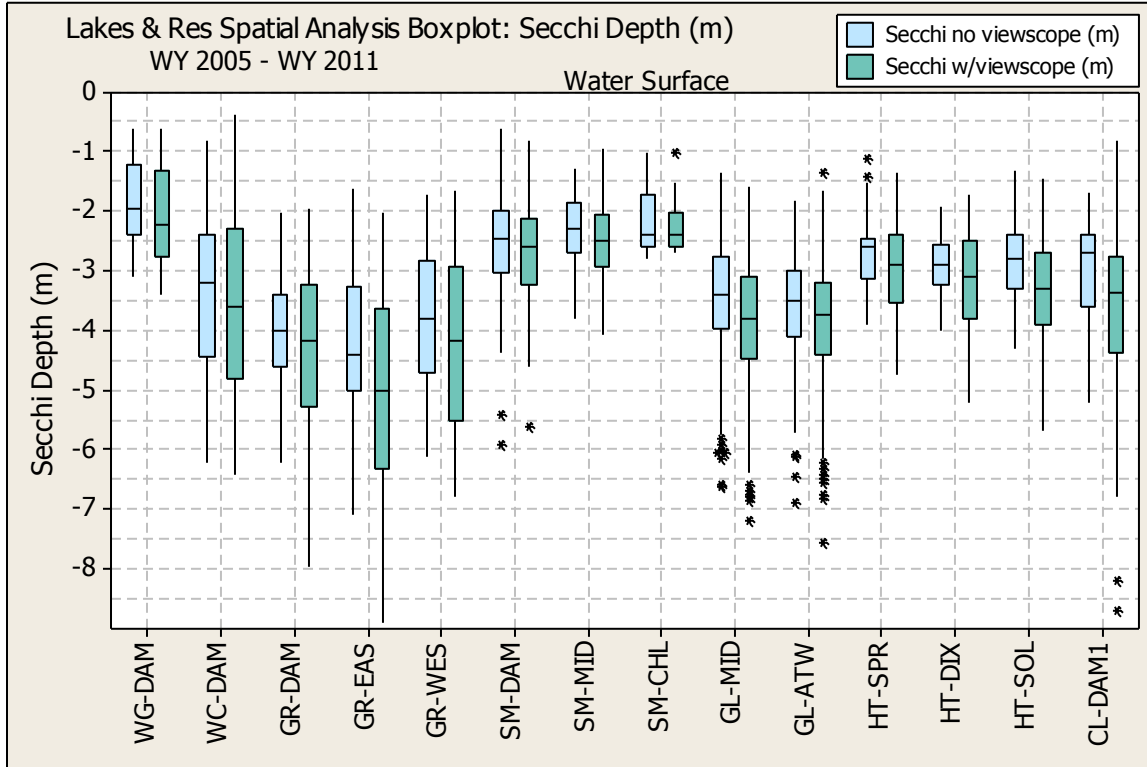
Figure E. 1 SECCHI DEPTH SPATIAL ANALYSIS BOX PLOT
