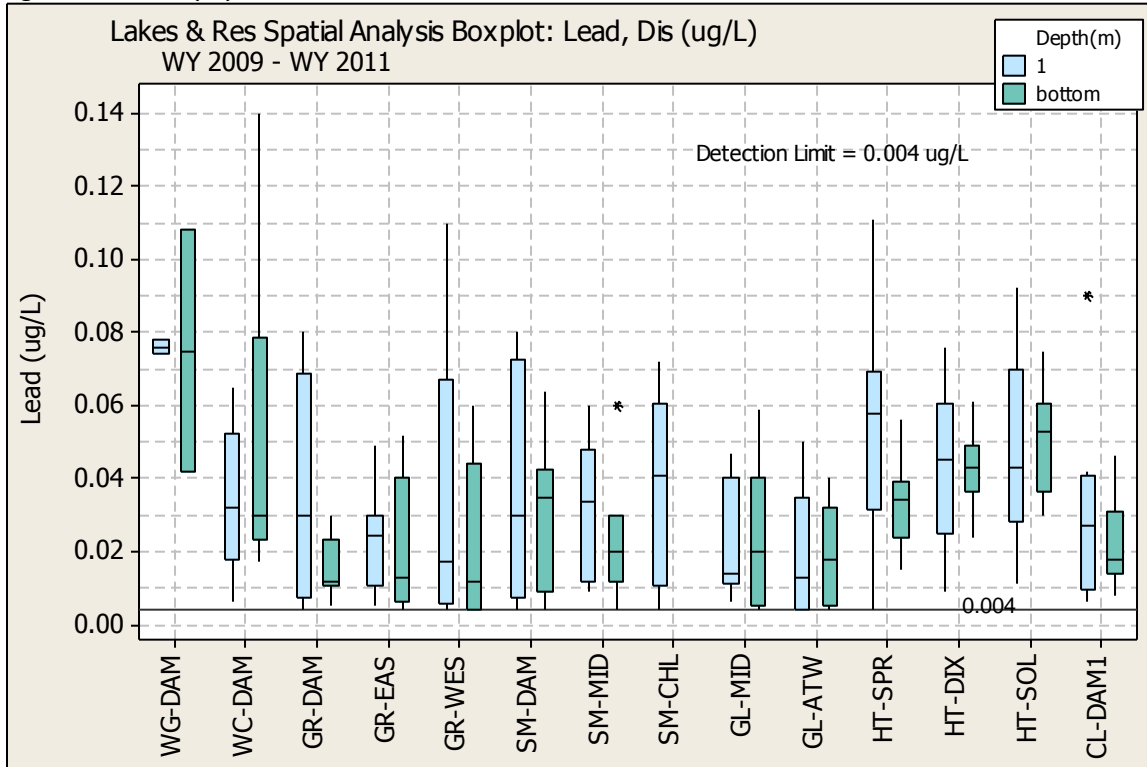
Figure E. 22 LEAD (Pb) SPATIAL ANALYSIS BOX PLOT
