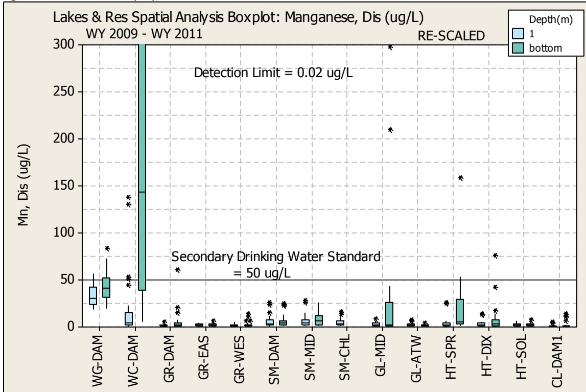
Figure E. 24 MANGANESE (Mn) SPATIAL ANALYSIS BOX PLOT -- RESCALED
