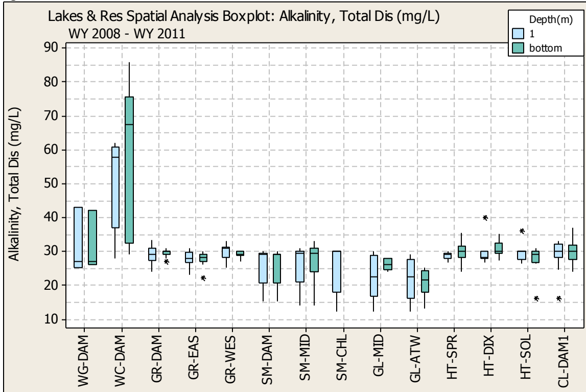
Figure E. 10 ALKALINITY SPATIAL ANALYSIS BOX PLOT
