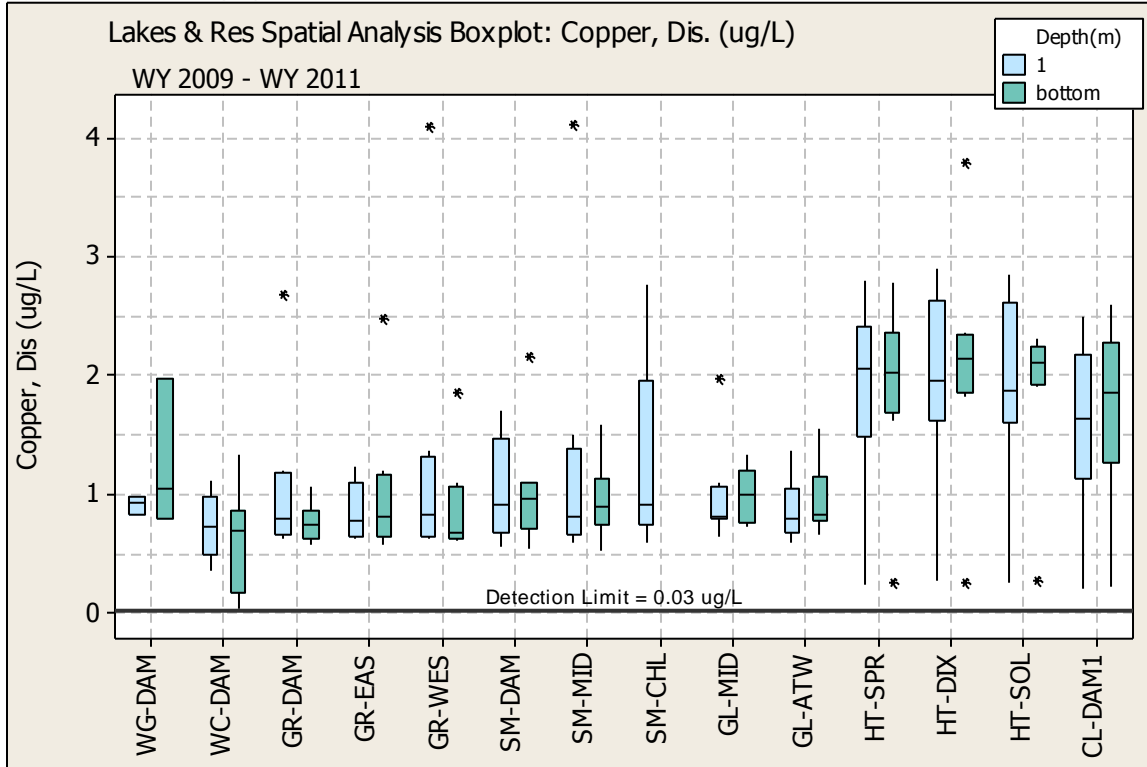
Figure E. 19 COPPER (Cu) SPATIAL ANALYSIS BOX PLOT
