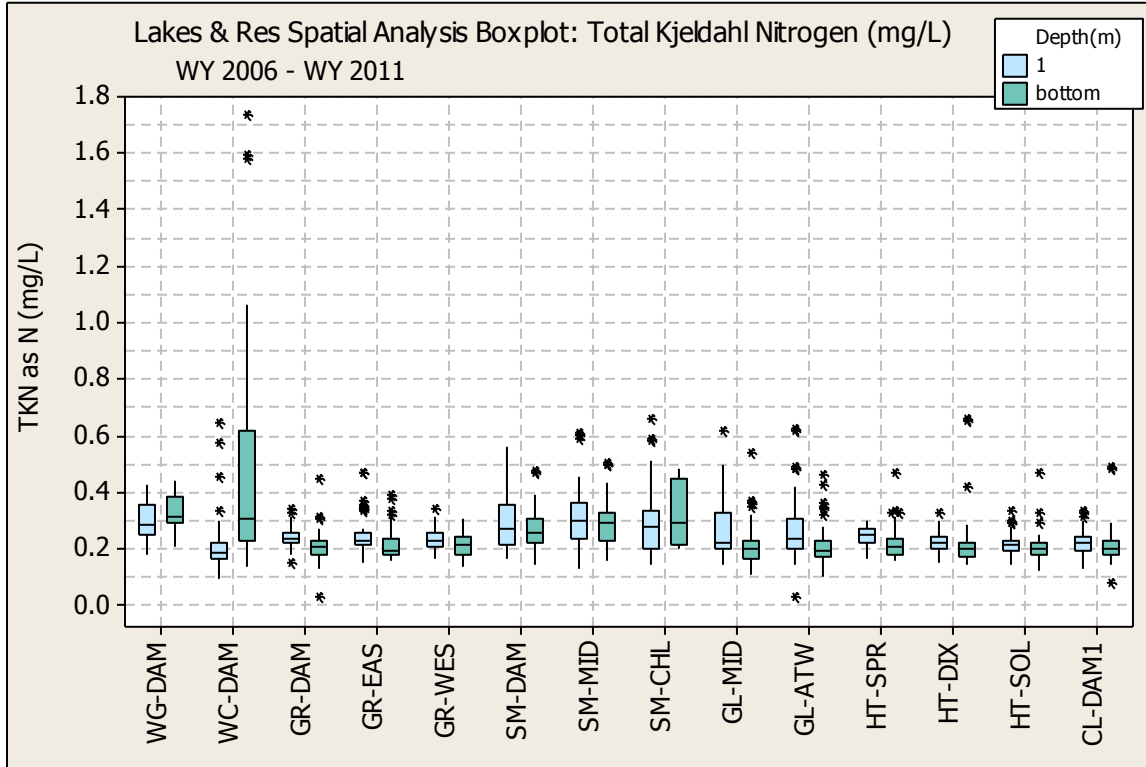
Figure E. 5 TOTAL KJELDAHL NITROGEN (TKN) SPATIAL ANALYSIS BOX PLOT
