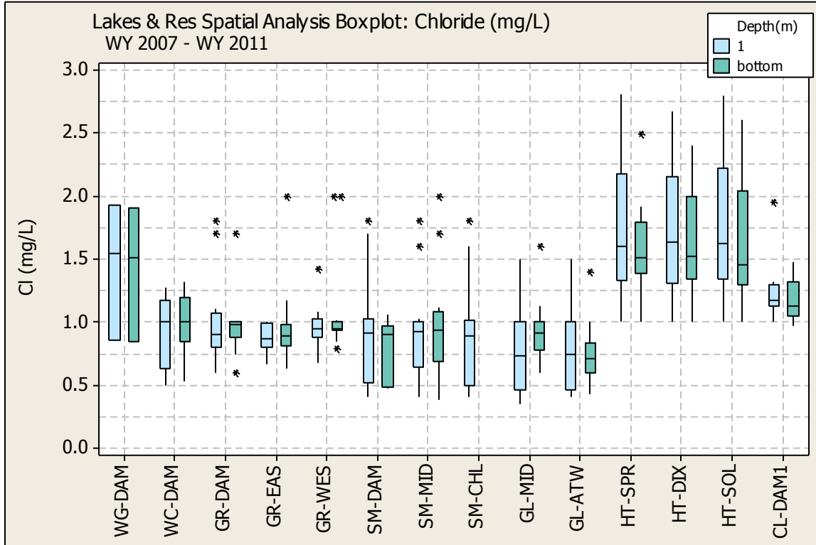
Figure E. 15 CHLORIDE SPATIAL ANALYSIS BOX PLOT
