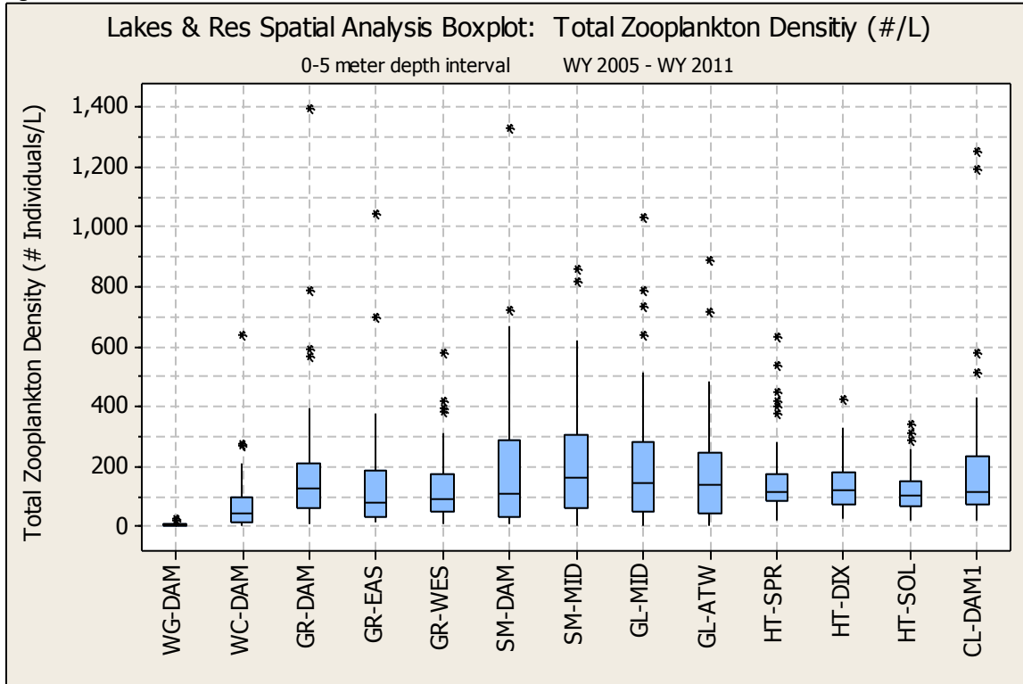
Figure E. 36 TOTAL ZOOPLANKTON DENSITY SPATIAL ANALYSIS BOX PLOT
