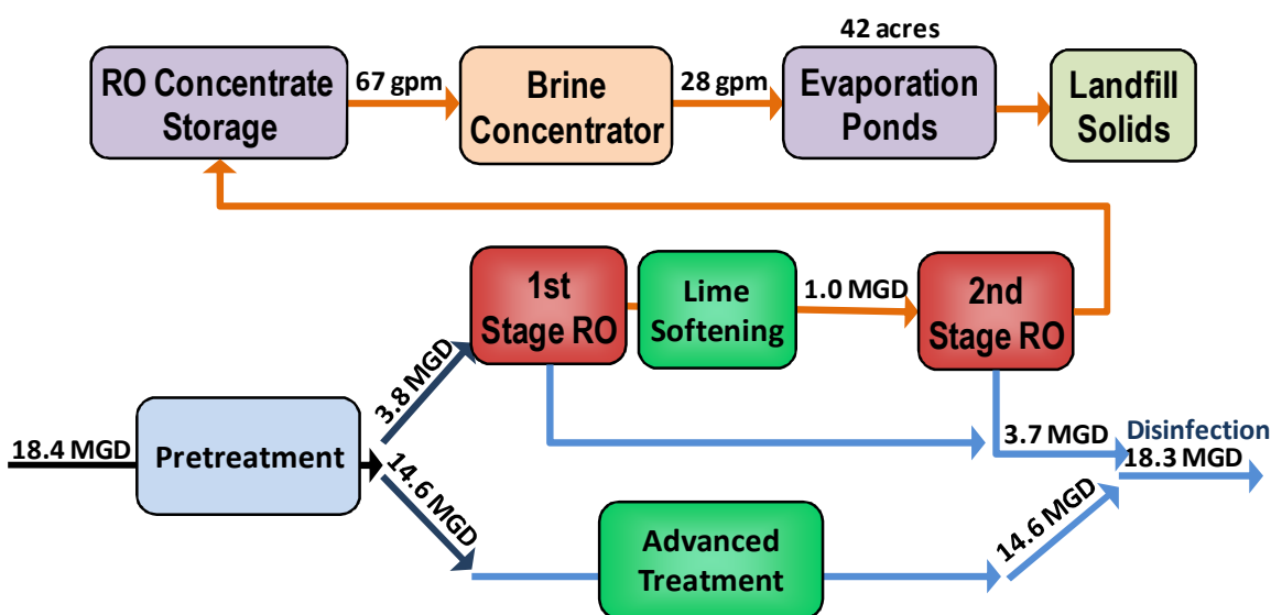
Figure 8. Option 1 – South Water Treatment Plant Schematic (Average Flow)
