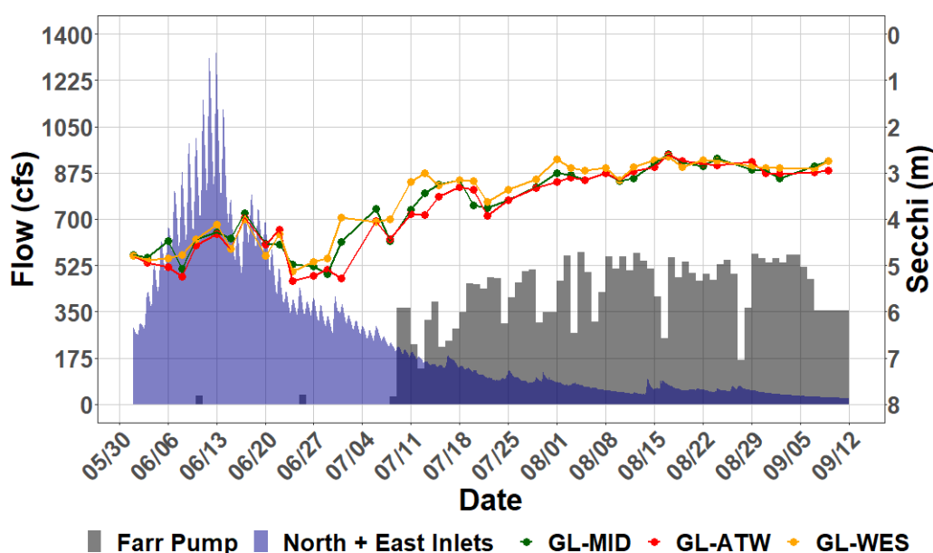
Figure 9: Grand Lake Secchi with Farr Pumping and North and East Inlets flows.
