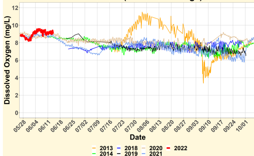
Shadow Mountain Dam Buoy Surface DO (0.5-1.5 m average)
