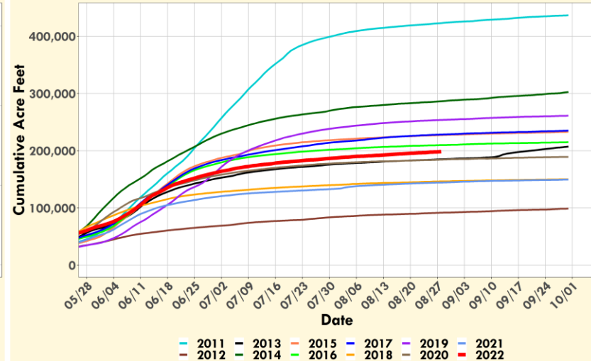
Cumulative Three Lakes Inflow Volumes by Year, May-Sep
