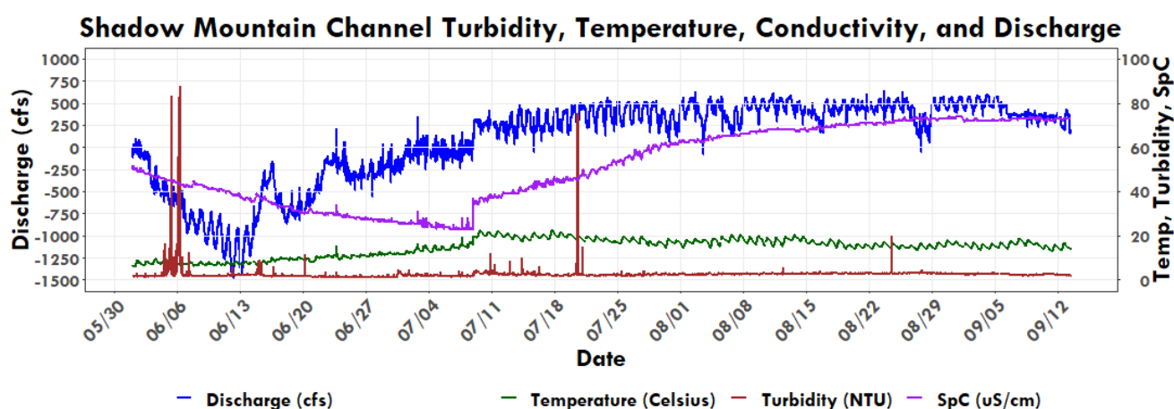
Figure 7: Turbidity, temperature, conductivity, and discharge at the Shadow Mountain Connecting Channel.
