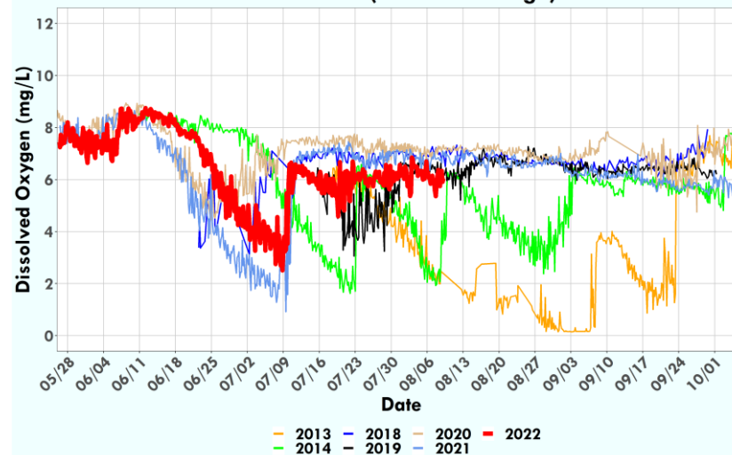
Shadow Mountain Dam Buoy Bottom DO (>6.8 m average)
