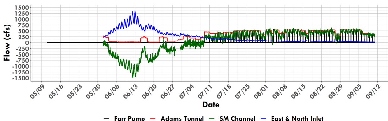
Figure 6: Farr pumping, Shadow Mountain Channel and Adams Tunnel Flows.
