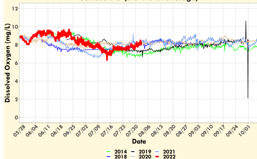
Shadow Mountain Mid Buoy Surface DO (0.5-1.5 m average)
