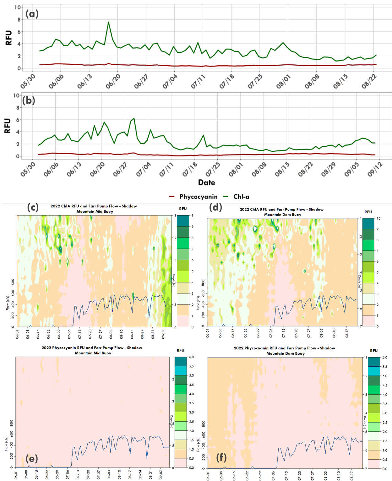
Figure 14: Chlorophyll a and phycocyanin data averaged between 0 and 2 m depths in time series form at SM-DAM (a) and SM-MID (b). Chlorophyll data in profile form at SM-MID (c) and SM-DAM (d). Phycocyanin data in profile form at SM-MID (e) and SM-DAM (f). Farr pumping rates are shown in (c), (d), (e), and (f).
