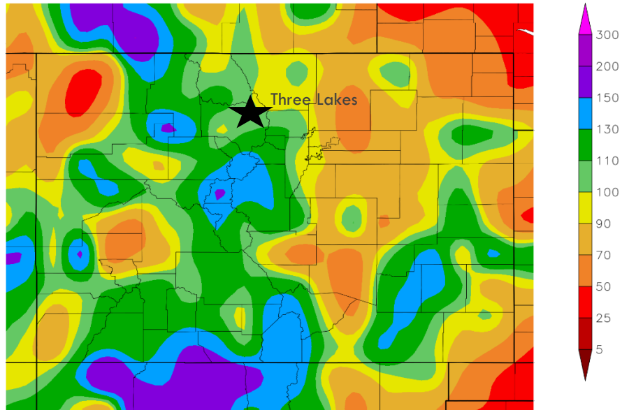
Figure 4: Percent of Normal Precipitation (%) 7/1/2022 - 9/30/2022 for Colorado.
