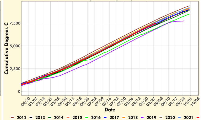
Cumulative Air Temp by Year, Apr-Sep
