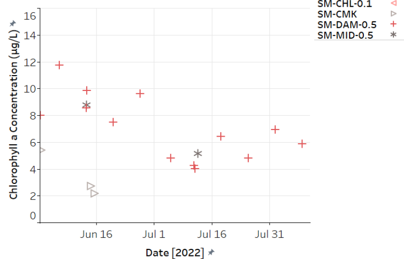
Chlorophyll a Concentrations in Grand Lake
