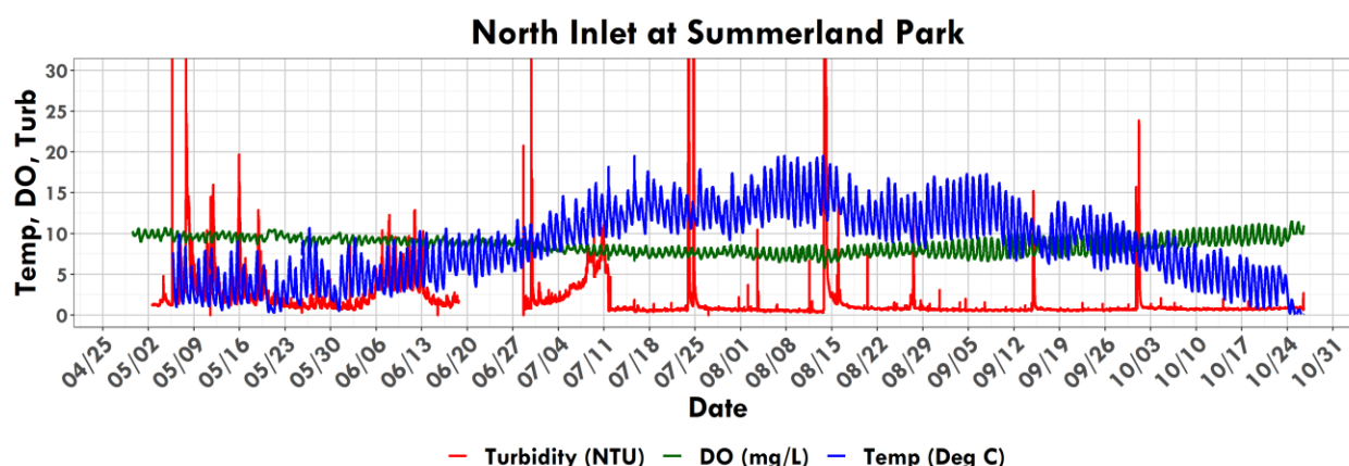
Figure 18: Temperature, DO, and Turbidity time series at North Inlet at Summerland Park (USGS).
