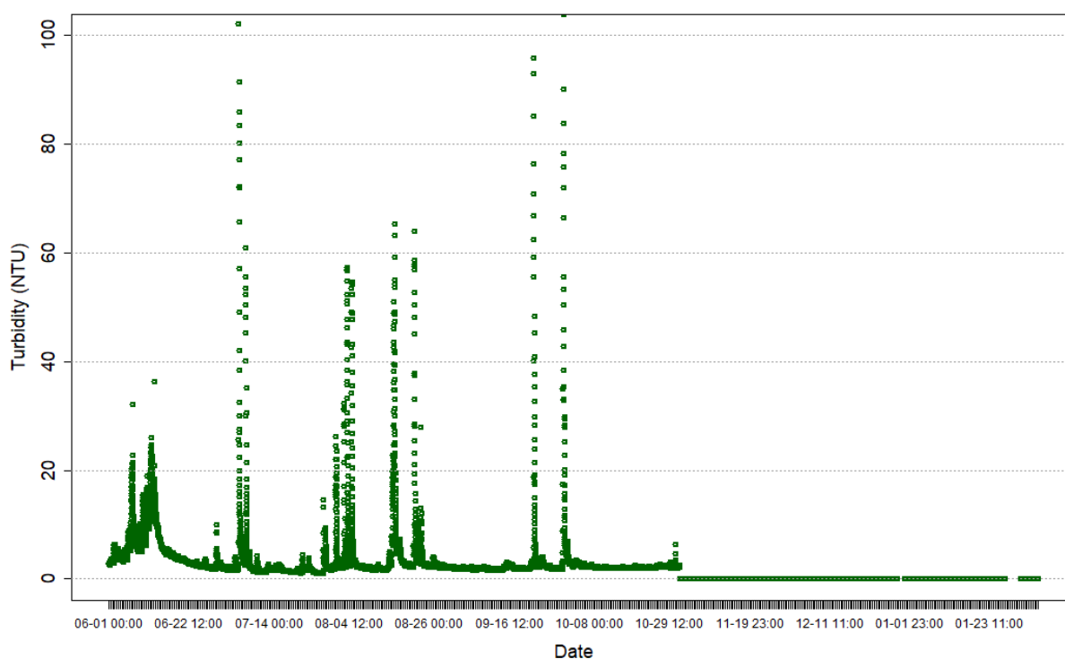
Figure 17: Provisional North Fork Turbidity time series.
