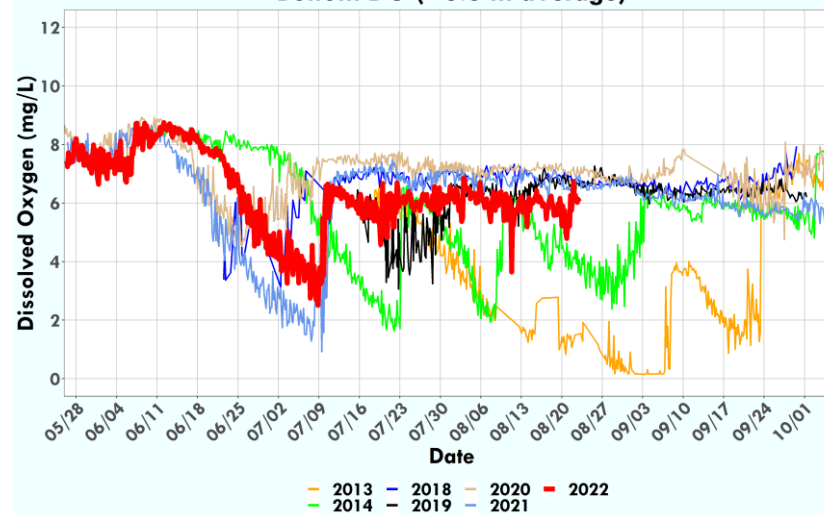
Shadow Mountain Dam Buoy Bottom DO (>6.8 m average)
