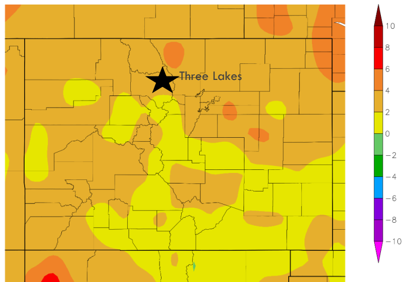
Figure 5: Departure from Normal Temperature (F) 7/1/2022 - 09/30/2022 for Colorado.
