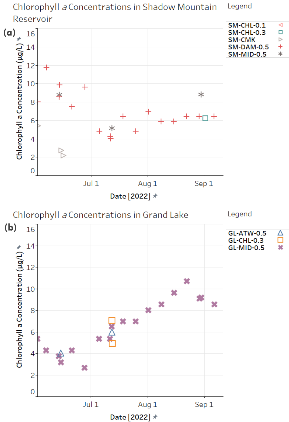
Figure 15: Chlorophyll a concentrations in Shadow Mountain Reservoir (a) and Grand Lake (b).
