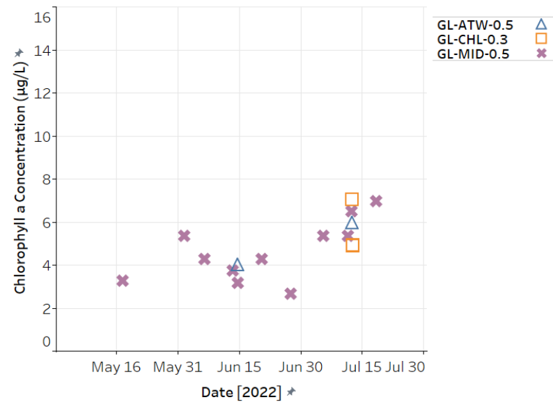
Chlorophyll a Concentrations in Grand Lake
