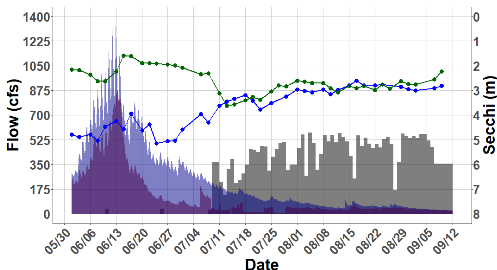
Figure 8: Shadow Mountain and Grand Lake Daily Average Secchi with Farr Pumping and Inflows.
