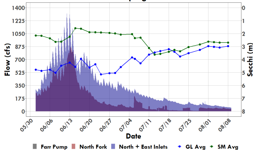
Shadow Mountain and Grand Lake Daily Avg Secchi with Farr Pumping and Inflows
