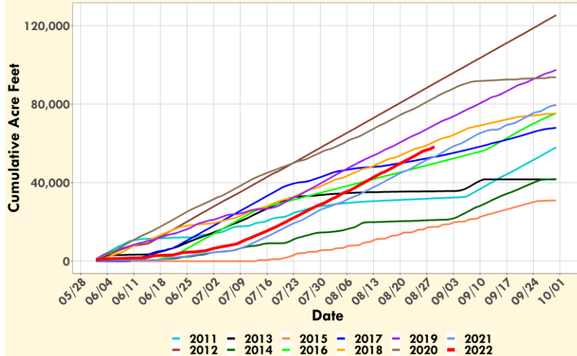
Cumulative Adams Tunnel Volumes by Year, Jun-Sep
