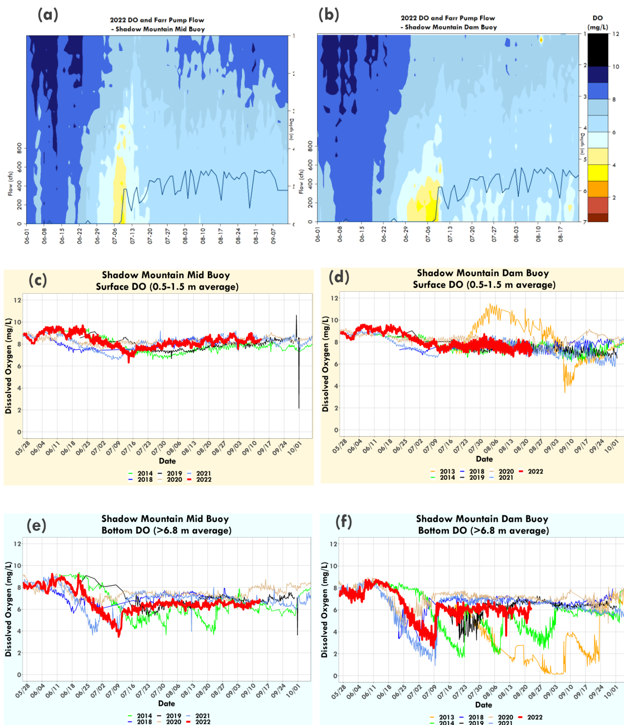
Figure 13: DO data in profile form at SM-MID (a), in profile form at SM-DAM (b), surface time series form at SM-MID (c), surface time series form at SM-DAM (d), bottom time series form at SM-MID (e) and bottom time series form at SM-DAM (f). Farr pumping rates are shown in (a) and (b).
