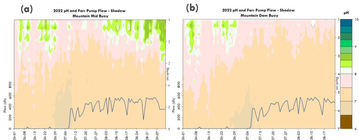
Figure 11: 2022 pH values (color) and daily Farr Pump flow (line) at SM-MID (a) and SM-DAM (b).
