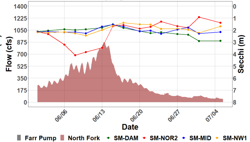
Shadow Mountain Secchi with Farr Pumping and North Fork flows
