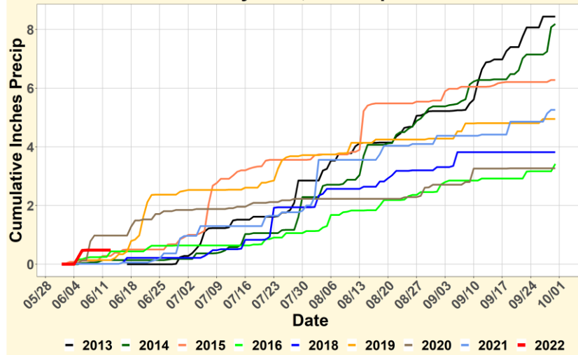
Cumulative NADP Precip by Year, Jun-Sep
