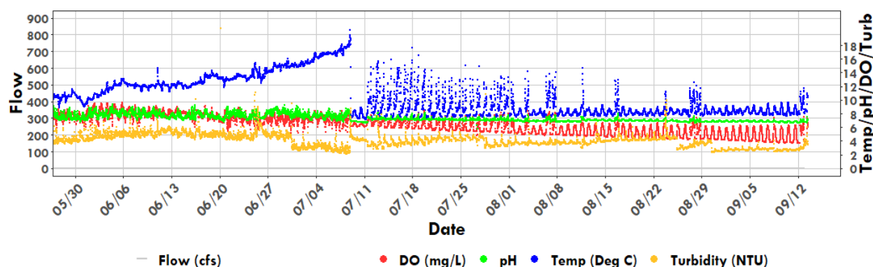
Figure 19: Discharge, temperature, pH, DO, and turbidity time series at GR-Pump.
