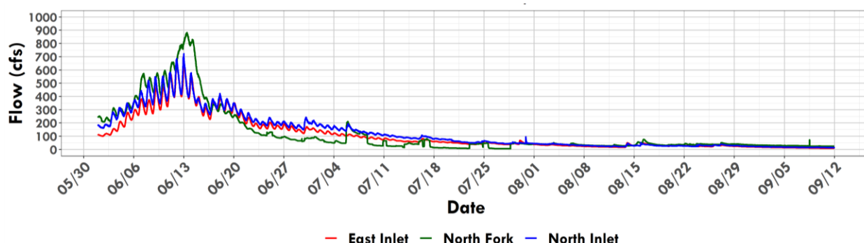
Figure 3: Grand Lake and Shadow Mountain Inflows: North Fork of the Colorado River, North, and East Inlets.
