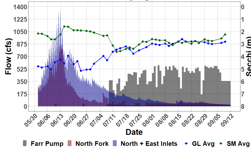
Shadow Mountain and Grand Lake Daily Avg Secchi with Farr Pumping and Inflows
